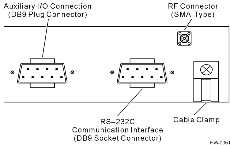
Figure 2-3 ASCII RS-232C Port
