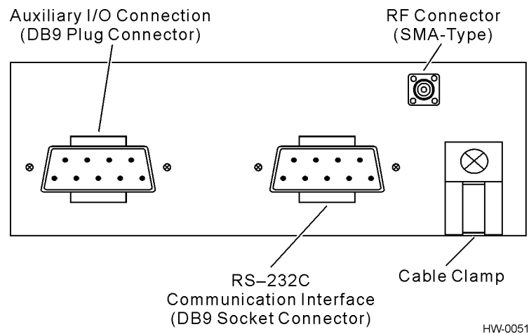
Figure 3-1 AI1401 Reader Connector Panel
